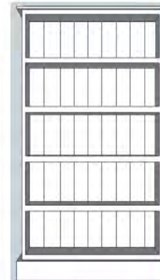
60 X 32 X 8 BOOKCASE SOM60328 h: 1524 w: 813 d: 203
