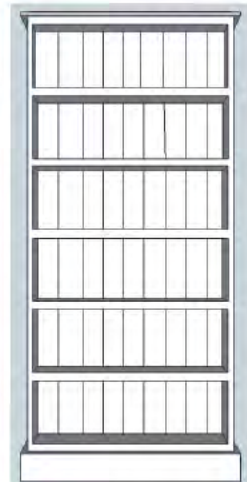
72 X 32 X 8 BOOKCASE SOM72328 h: 1828 w: 813 d: 203
